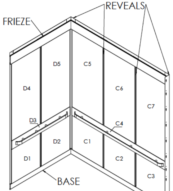
ISOMETRIC
